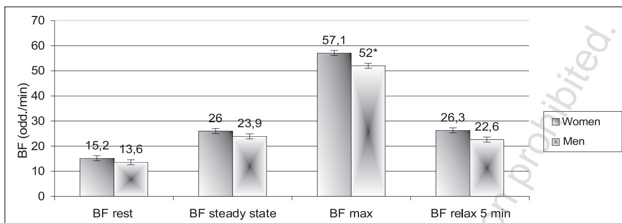
Fig.4. Breathing frequency(BF odd./min) in the studied female and male judoists in test exertion ( p<0.05^* )
