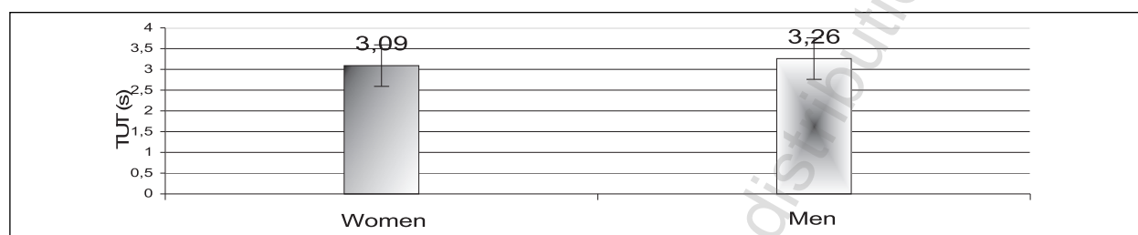
Fig. 9. Mean values of the time of maintaining maximal power [TUT(s)] in the studied female and male judoists obtained during Wingate test
